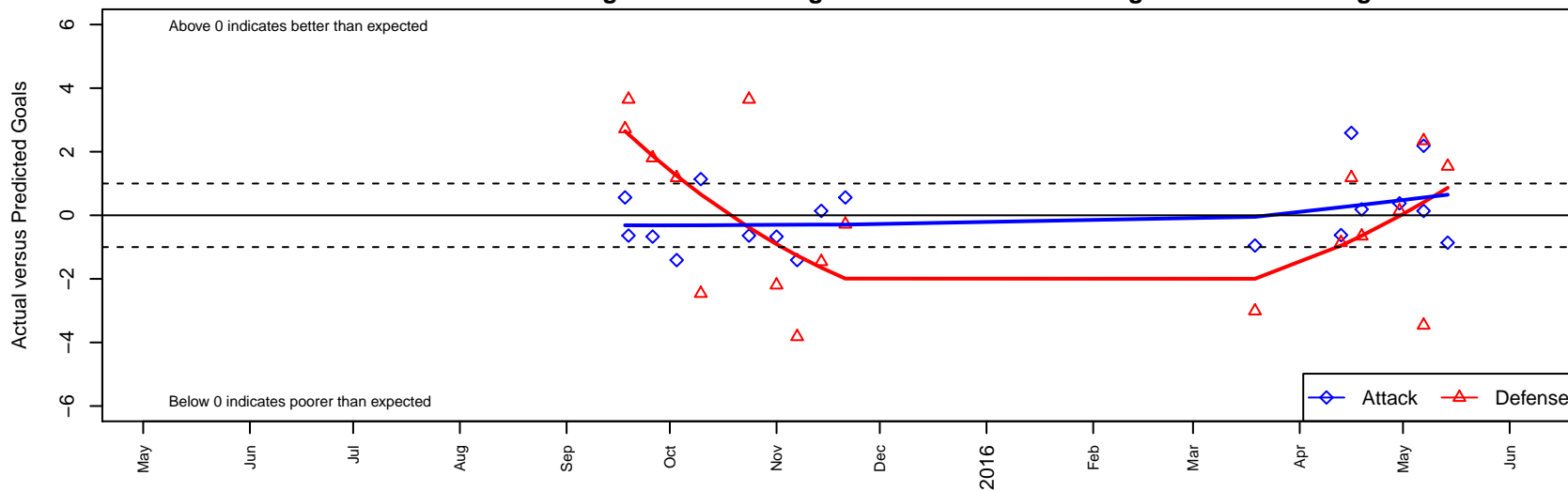
FC Spokane Grey 2002B Dots are actual minus expected GF (blue circles) and GA (red triangles). Blue line is smoothed change in attack strength. Red is smoothed change in defense strength.
